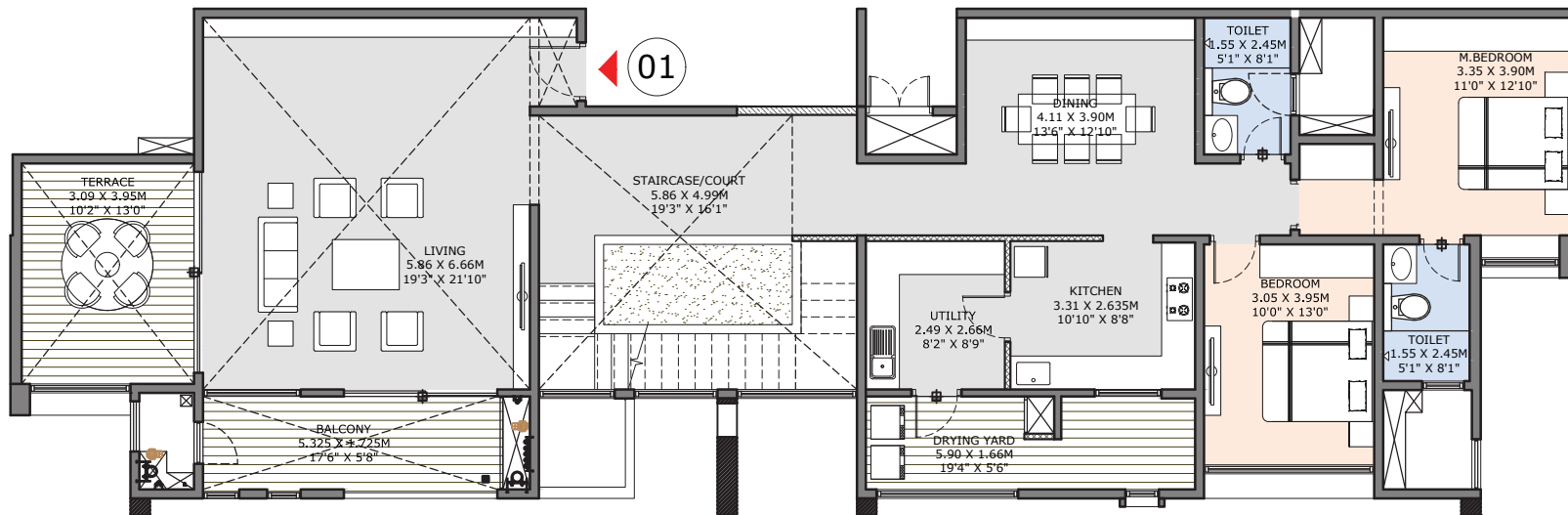
LOWER LEVEL PLAN
